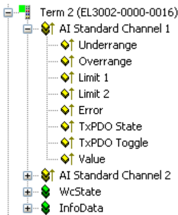
Fig. 195: Element-orientated process data of the EL30xx-0000-0016
