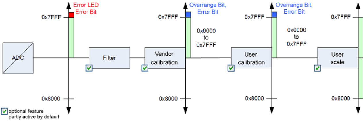
Fig. 204: Data flow with correction calculation - EL301x, EL304x
