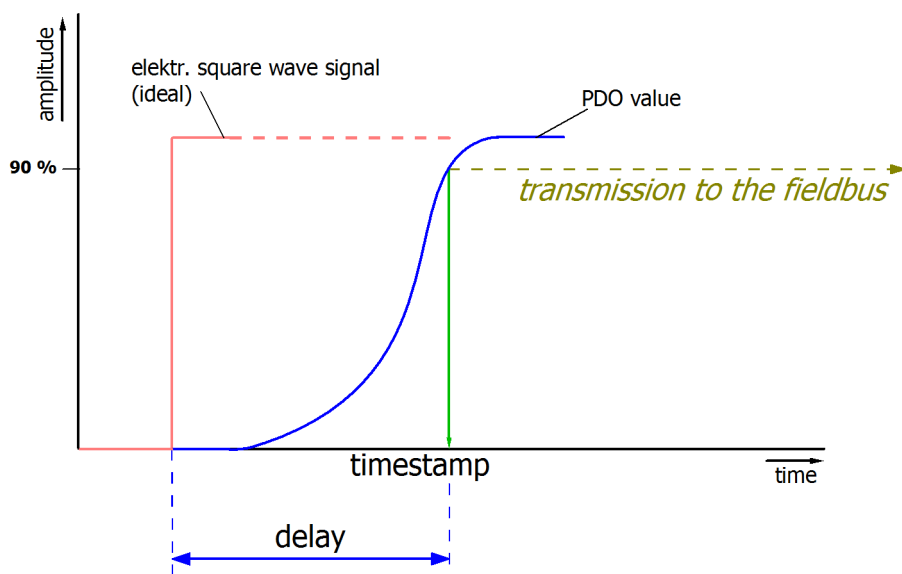
Fig. 228: Diagram signal delay (step response)
