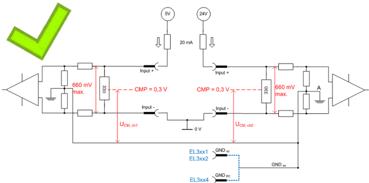
Fig. 75: Example 1: low-side measurement
