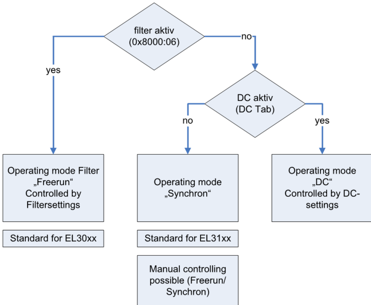
Fig. 199: Relationship of operating modes
