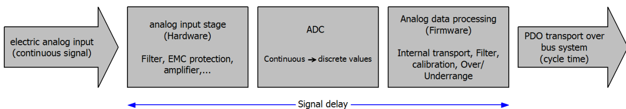
Fig. 227: Signal processing analog input
