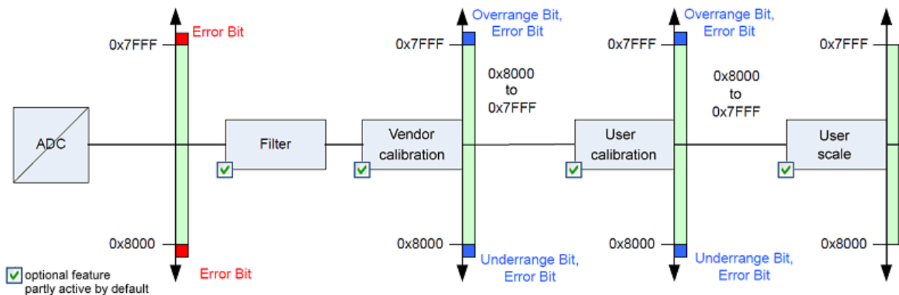
Fig. 203: Data flow with correction calculation - EL300x
