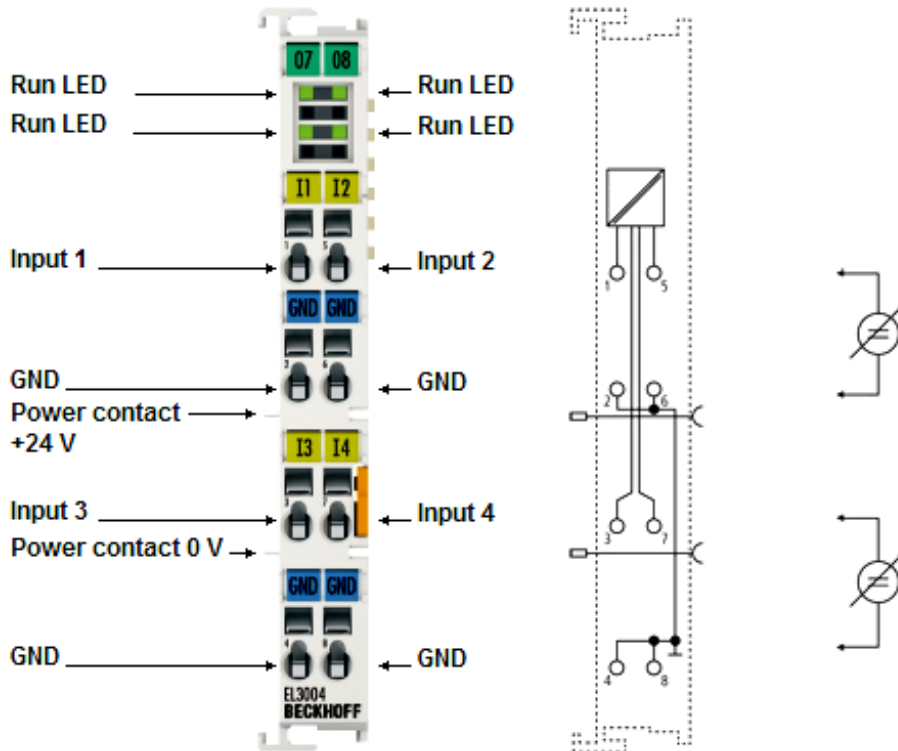
Fig. 9: LED EL3004
