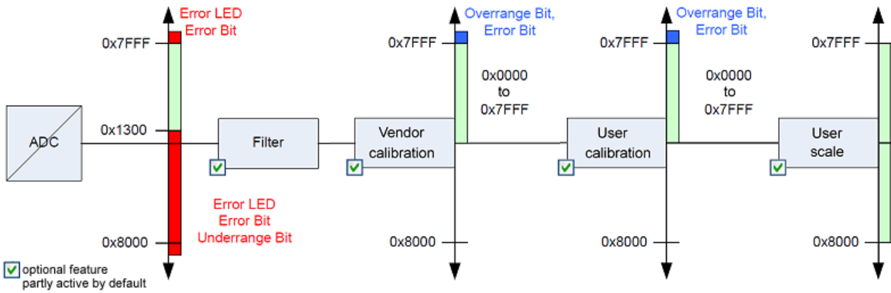
Fig. 205: Data flow with correction calculation - EL302x, EL305x
