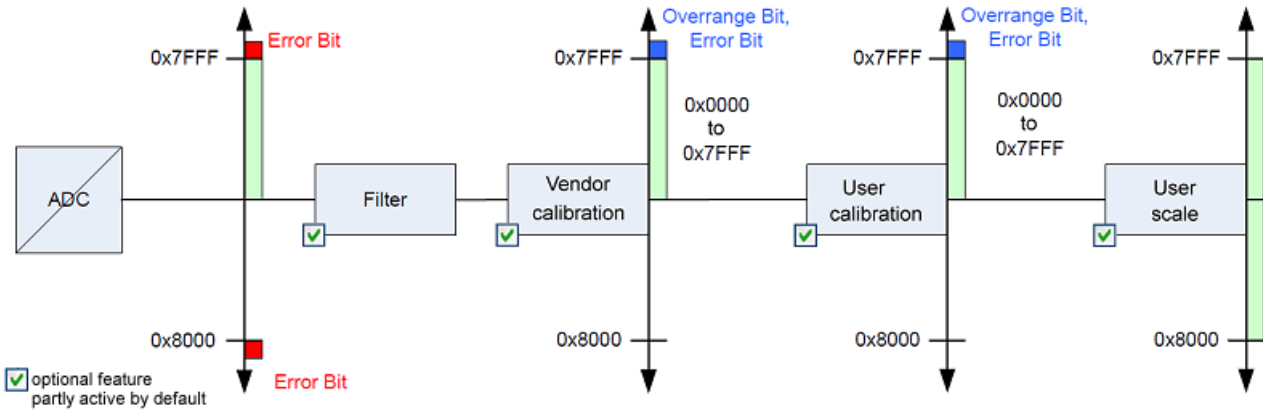
Fig. 206: Data flow with correction calculation - EL306x
