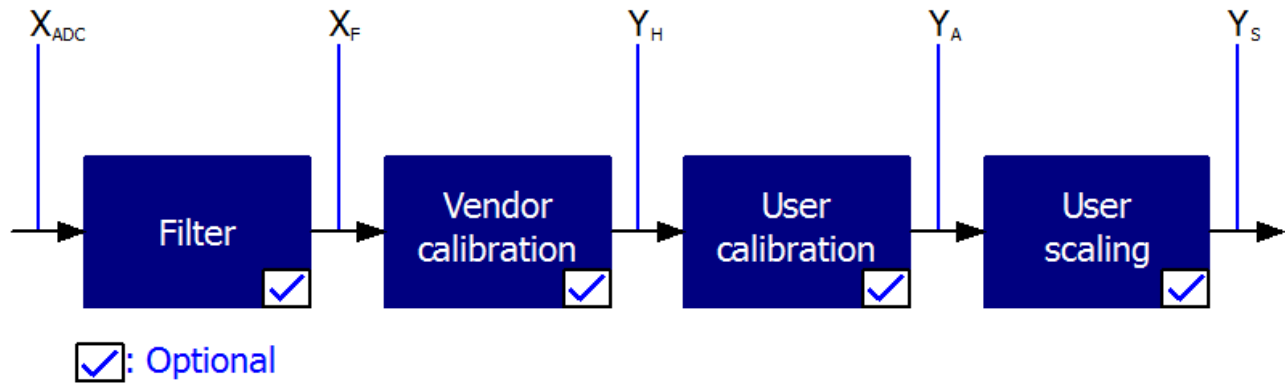
Fig. 213: Calculation of process data
