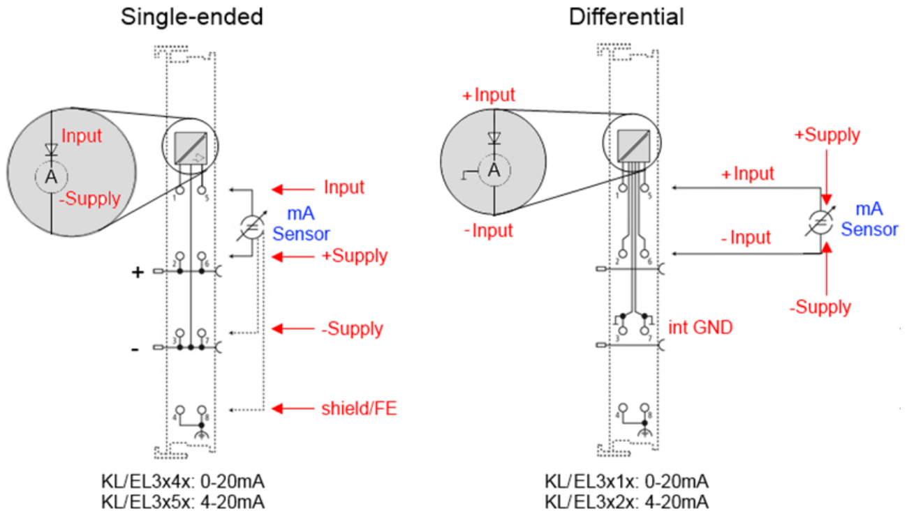
Fig. 223: Connection of externally supplied sensors
