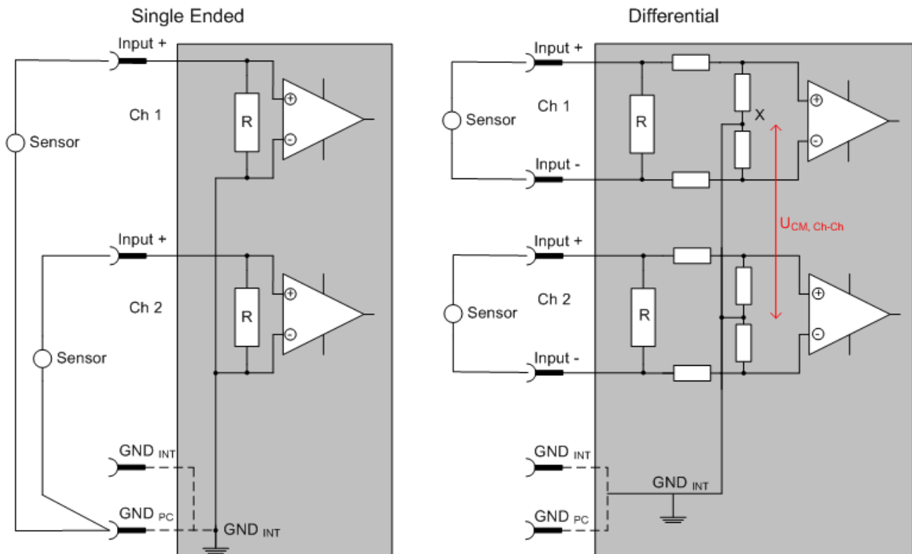
Fig. 221: SE and DIFF module as 2-channel version
